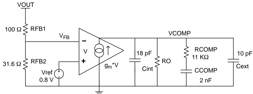
Figure 34. Example of the Feedback Compensation Network
